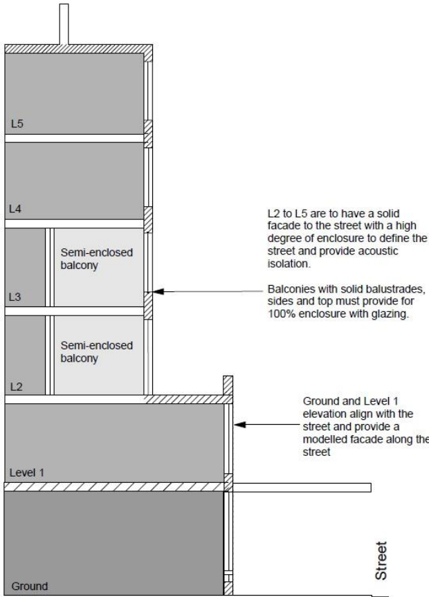
Figure 28 Façade section
