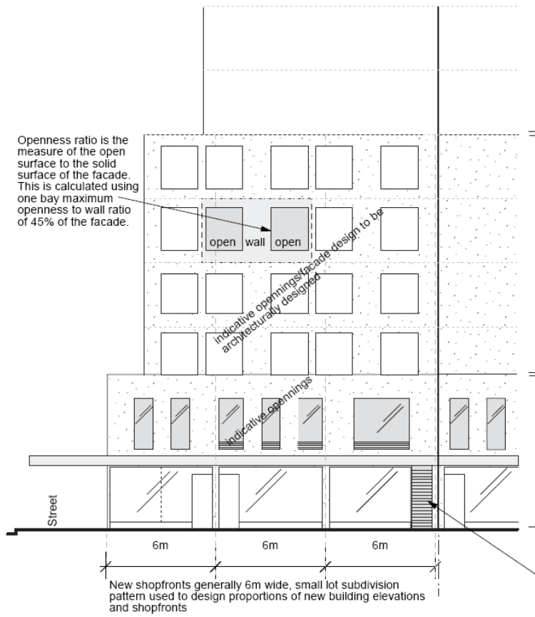
Figure 27 Elevations
