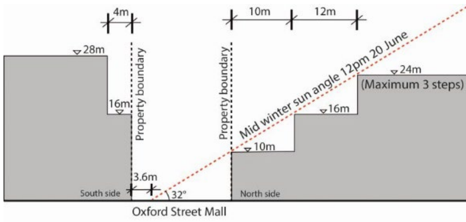
Figure 35 Street frontage Type A – Oxford Street Mall
